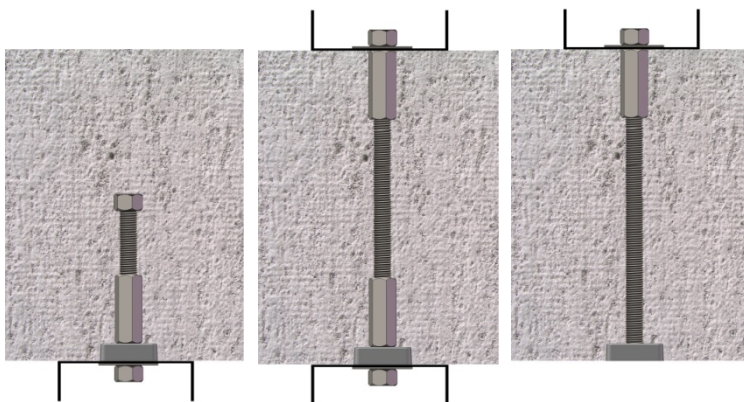
BELOW SLAB ONLY CONNECTION ABOVE & BELOW SLAB CONNECTIONS ABOVE SLAB ONLY CONNECTION
